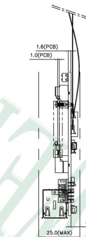
Detail SBC Board Scale 1X
